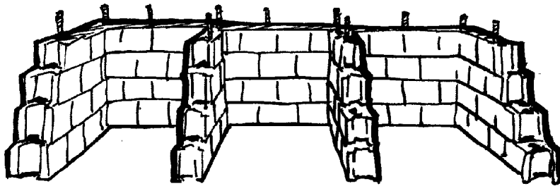
b. Cement block three-bin composting unit.
